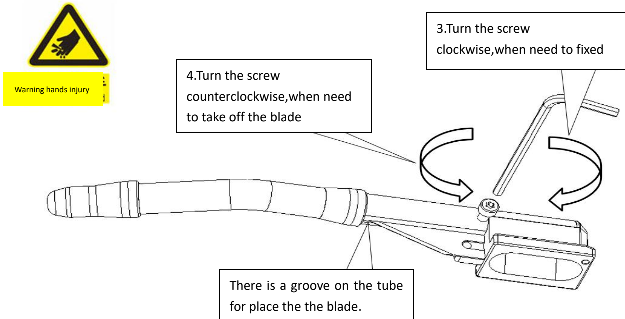
Pic 6(blade replace and install instruction diagram 3)
